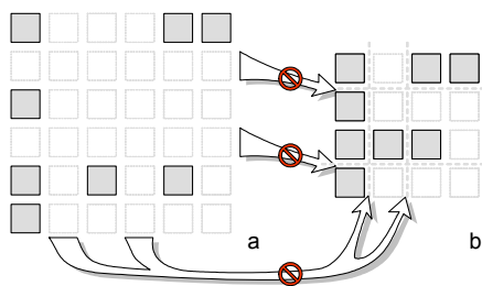
Figure 5: Drag-and-pop computes tip icon layouts (a) by snapping icons to a grid and then (b) removing empty rows and columns.
